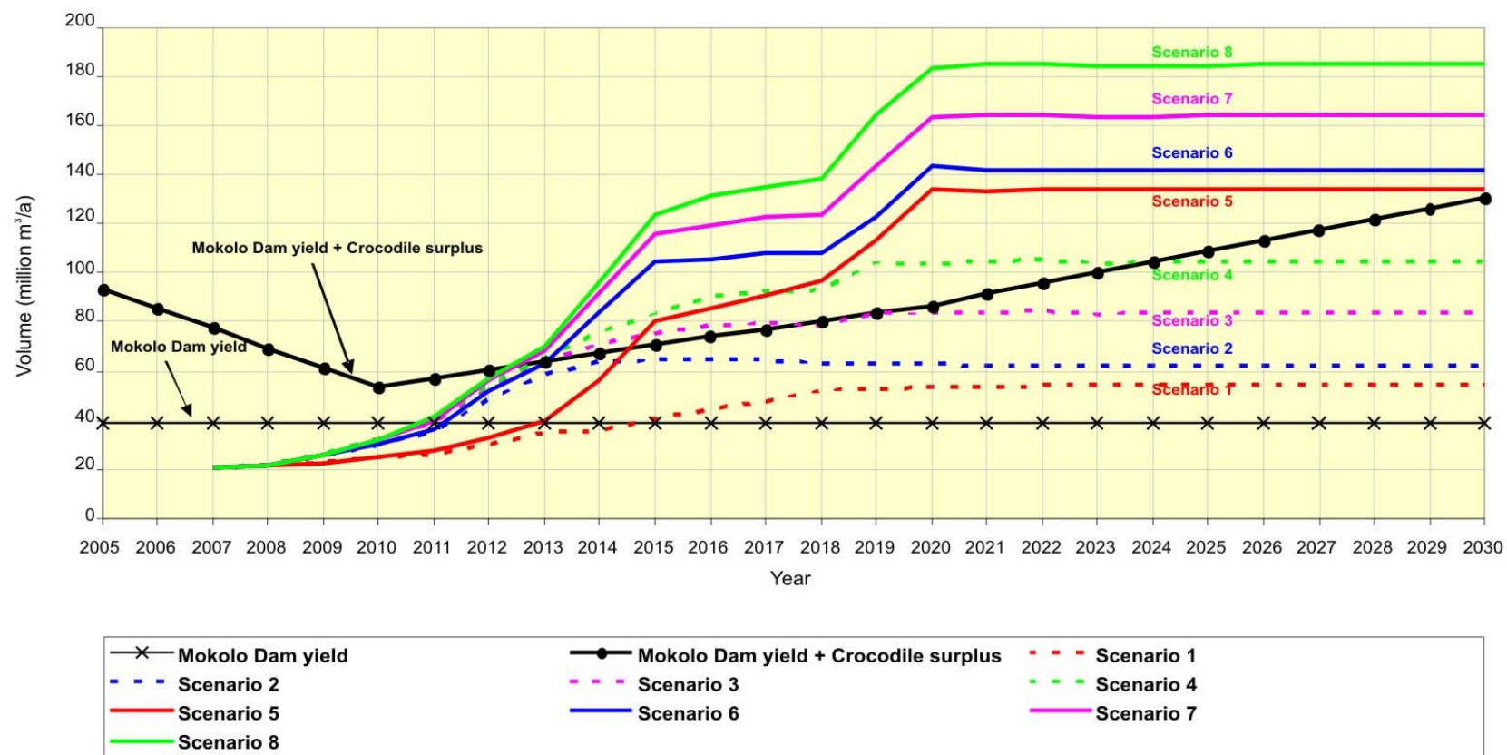
Figure A-2: Water Balance at Lephalale: Base Population, Medium Efficiency (DWA, 2008c)
